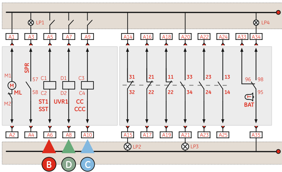
Connection scheme RTC (BLOCK A) Anschlüsse RTC (BLOCK A) Schema connessione RTC (Morsettiara A)
