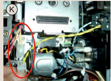
Plug connection CCC-EC switch Steckerverbindung CCC-EC-Schalter Connessione spinotto CCC-contatto CE
