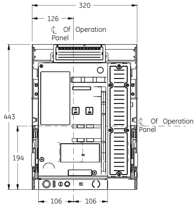
Front view 4pole
