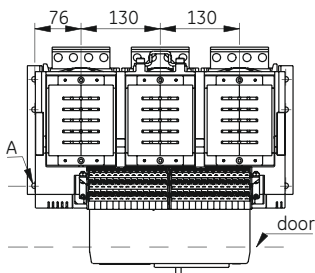
Top view 3pole
