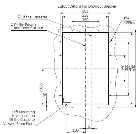
Door Cut-out
