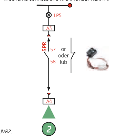
... Connection scheme RTC (BLOCK A) ... Anschlüsse RTC (BLOCK A) ... Schema connessione RTC (MORSETTIERA A)
