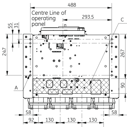
Top view 3pole
