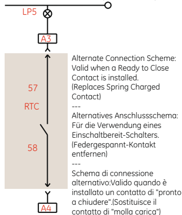
Connection scheme RTC (BLOCK A) Anschlüsse RTC (BLOCK A) Schema connessione RTC (Morsettiara A)
